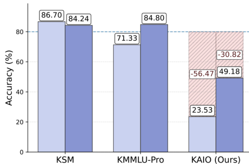
Figure 1: Accuracy of DeepSeek-R1 (light purple) and Gemini-2.5-Pro (dark) on KSM, KMMLU-Pro, and KAIO.
